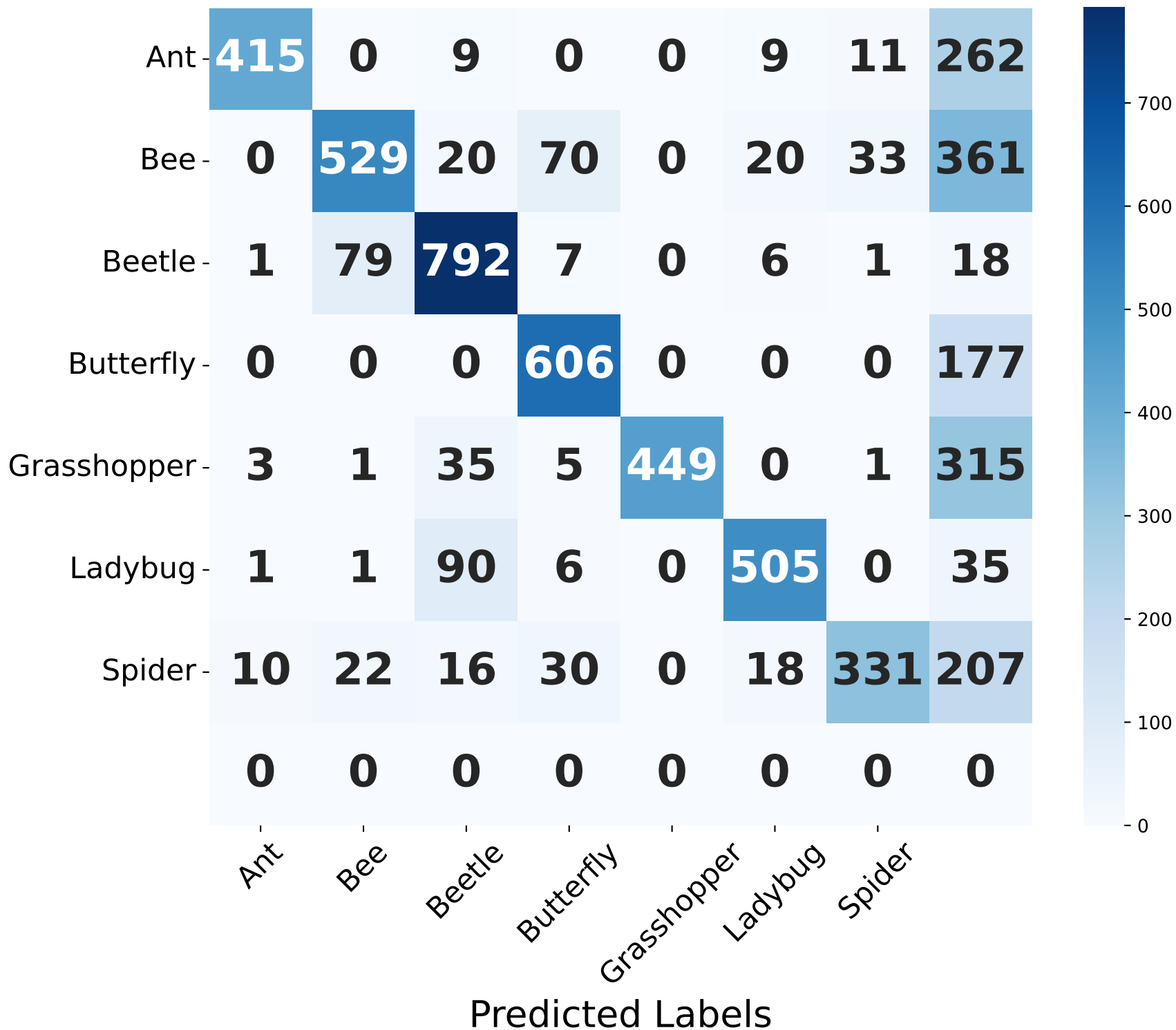
Confusion Matrix: Full iNat (LoRA)
